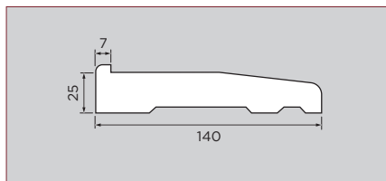
Composite Sill 140mm x 25mm x 3.1m Colour: Brown Part Code: 1.10.0978.3100.10
