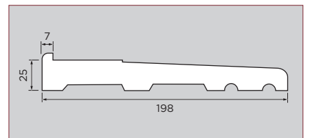
Composite Sill 198mm x 25mm x 3.1m Colour: Brown Part Code: 1.10.0970.3100.10
