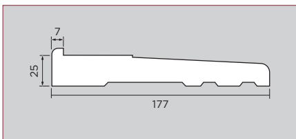
Composite Sill 177mm x 25mm x 3.1m Colour: Brown Part Code: 1.10.0971.3100.10
