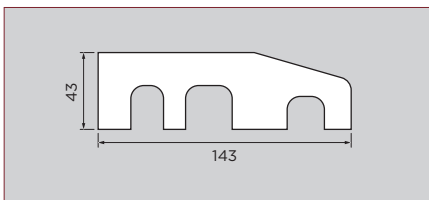
Composite Sill 143mm x 43mm x 3.1m Colour: Brown Part Code: 1.10.0972.3100.10
