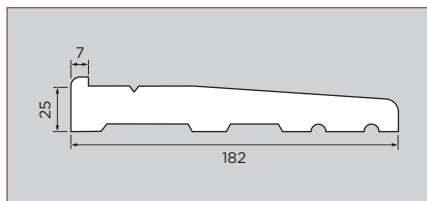
Composite Sill 182mm x 25mm x 3.1m Colour: Brown Part Code: 1.10.0977.3100.10
