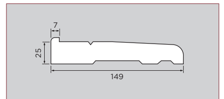
Composite Sill 149mm x 25mm x 3.1m Colour: Brown Part Code: 1.10.0975.3100.10
